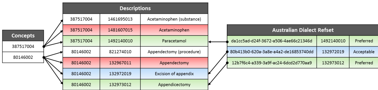
Figure 9: Relationship between the concepts, descriptions and Language type reference set
