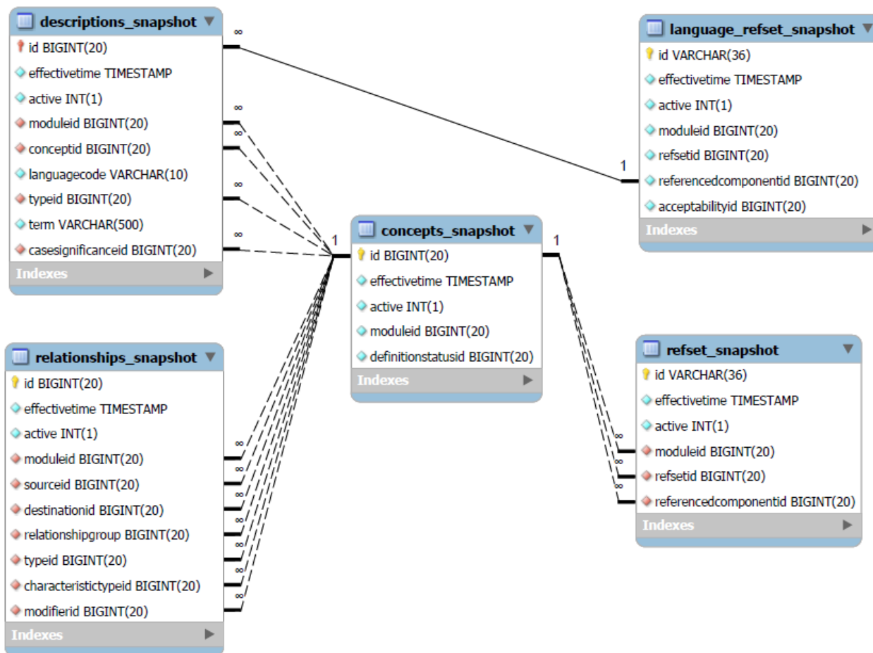
Figure 19: Entity-relationship diagram for sample schema
