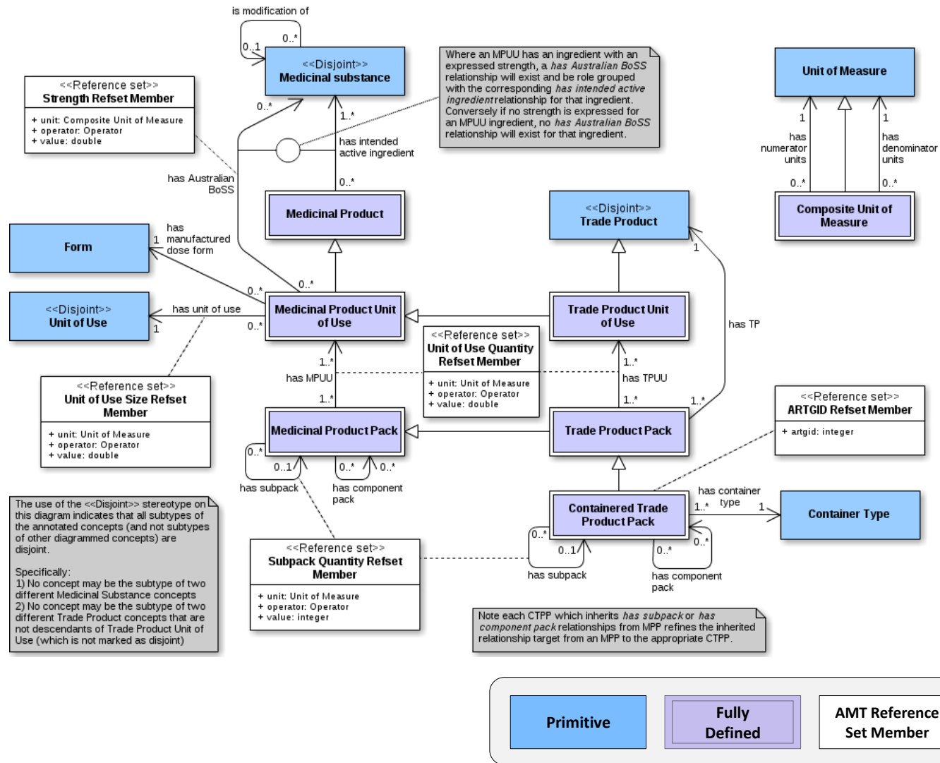
Figure 2: The AMT concept model
