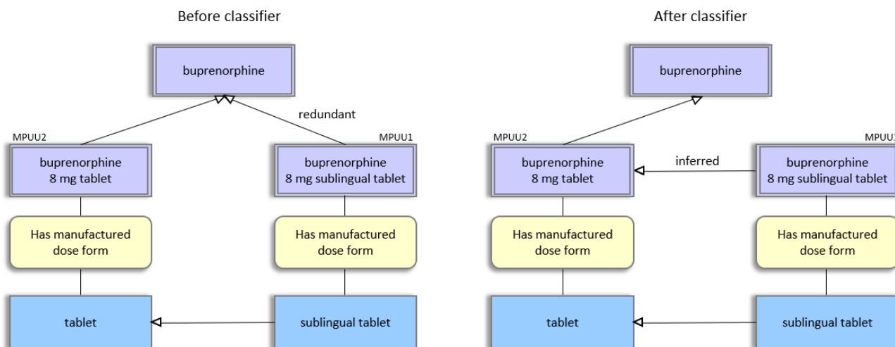
Figure 17: An example of IS A relationships between MPUU and MP using current AMT editorial rules before using a description logic classifier (left) and after (right)
