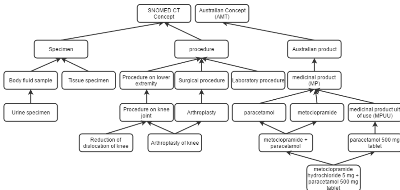
Figure 1: Example conceptual view of the SNOMED CT-AU hierarchy (not all intermediate concepts are shown)
