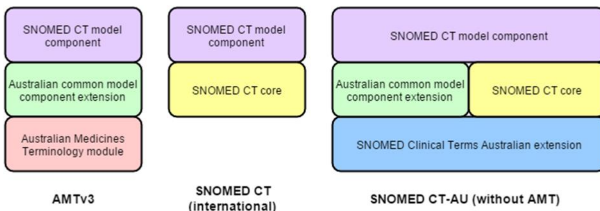
Figure 25: Release modules in terminology releases
