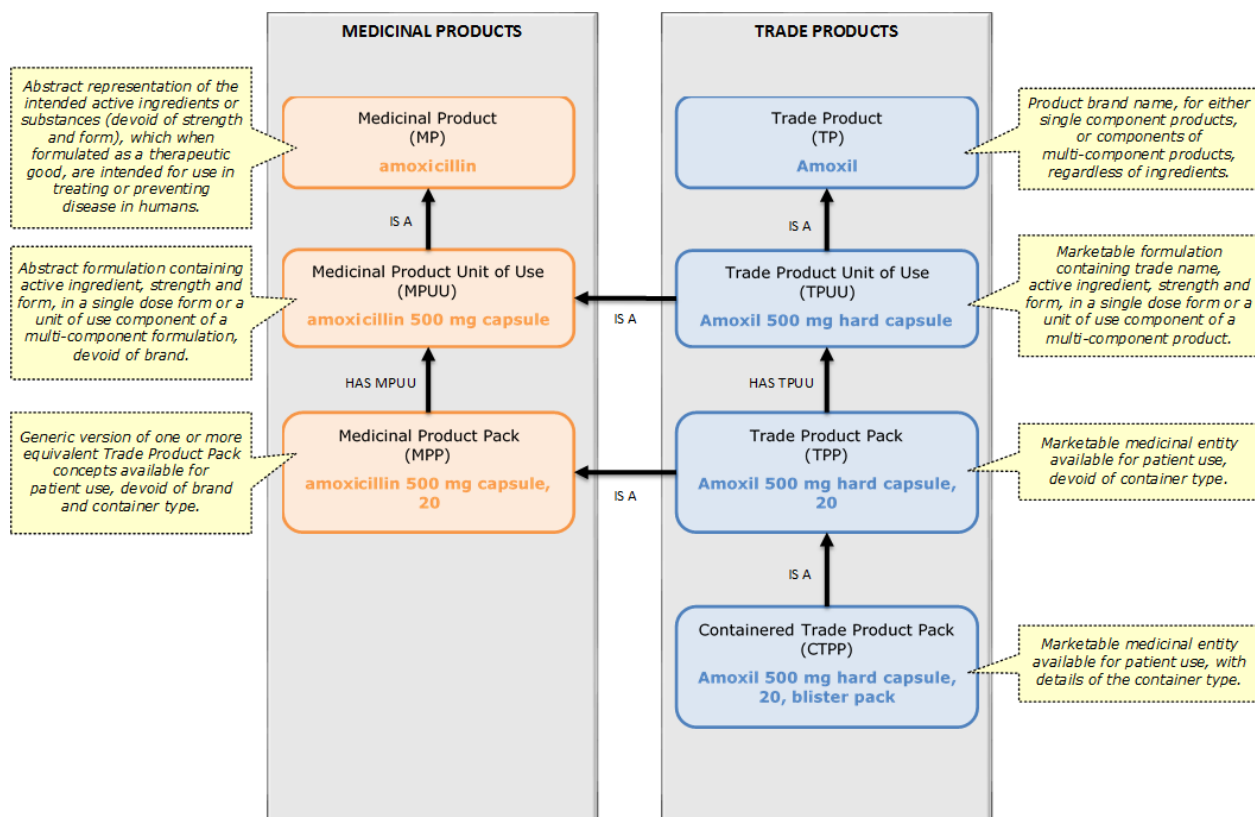
Figure 3: Seven notable concepts of the AMT and their definitions
