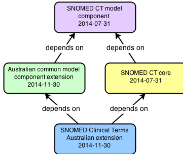
Figure 26: SNOMED CT AU module dependency as of November 2014
