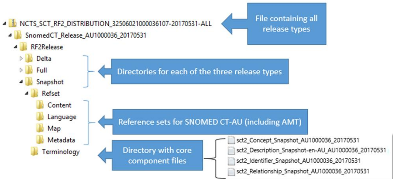
Figure 4: Directory layout of release bundle
