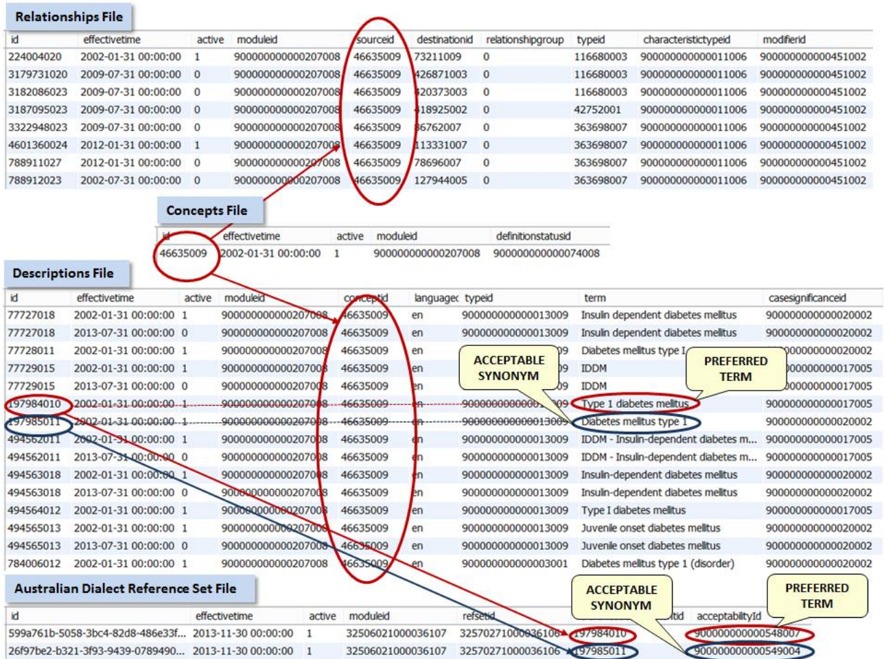
Figure 8: Retrieving the Preferred Term and acceptable Synonym for concept 46635009
