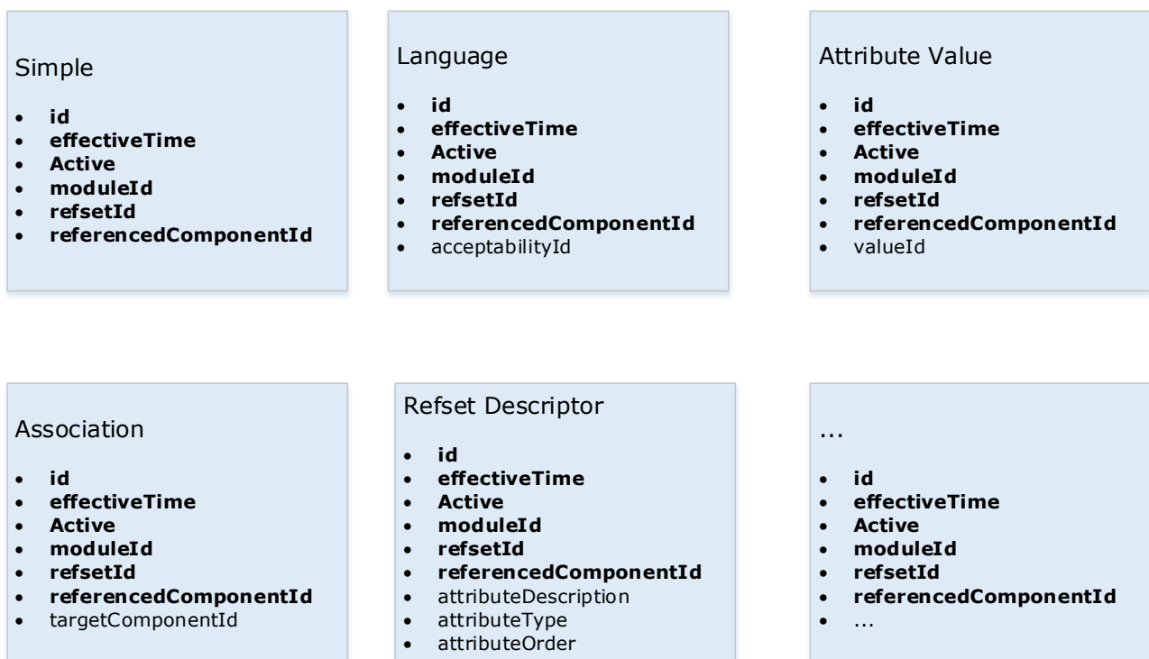
Figure 7: Common attributes of various reference sets
