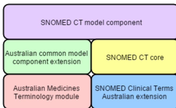
Figure 27: Module composition for SNOMED CT AU combined with the AMT
